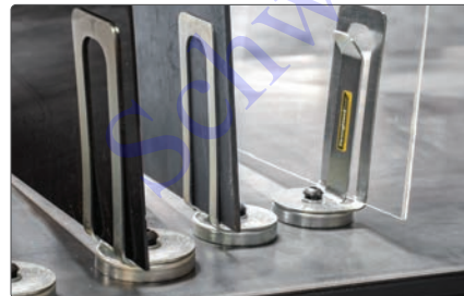
140 mm H "clip style" Holders support panel thicknesses up to 10 mm.
